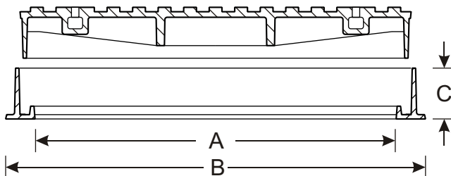
SECTIONAL VIEW OF COVER & FRAME
