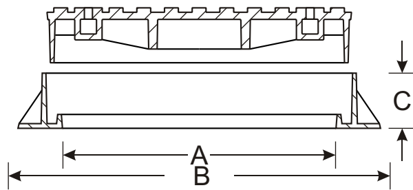
SECTIONAL VIEW OF COVER & FRAME
