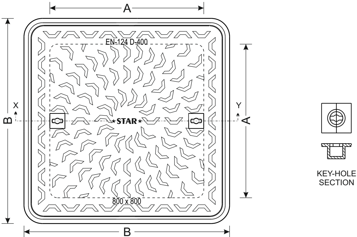
TOPVIEW OF COVER
