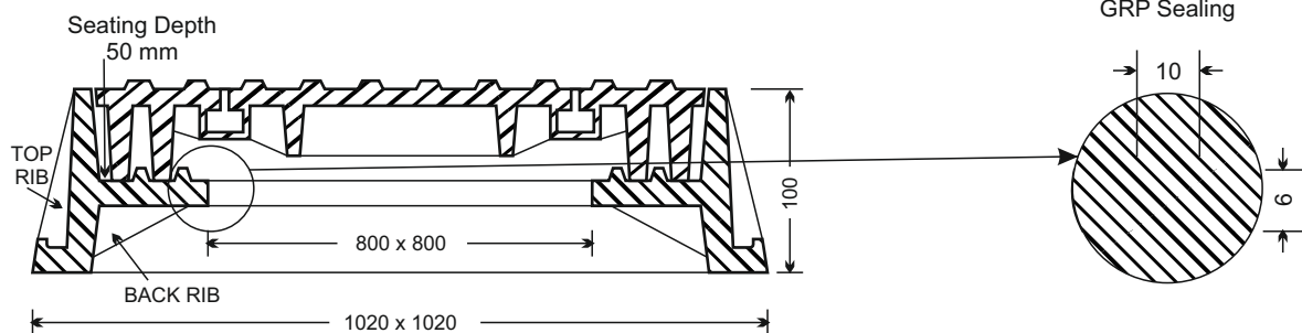
SECTIONALVIEW OF COVER & FRAME
