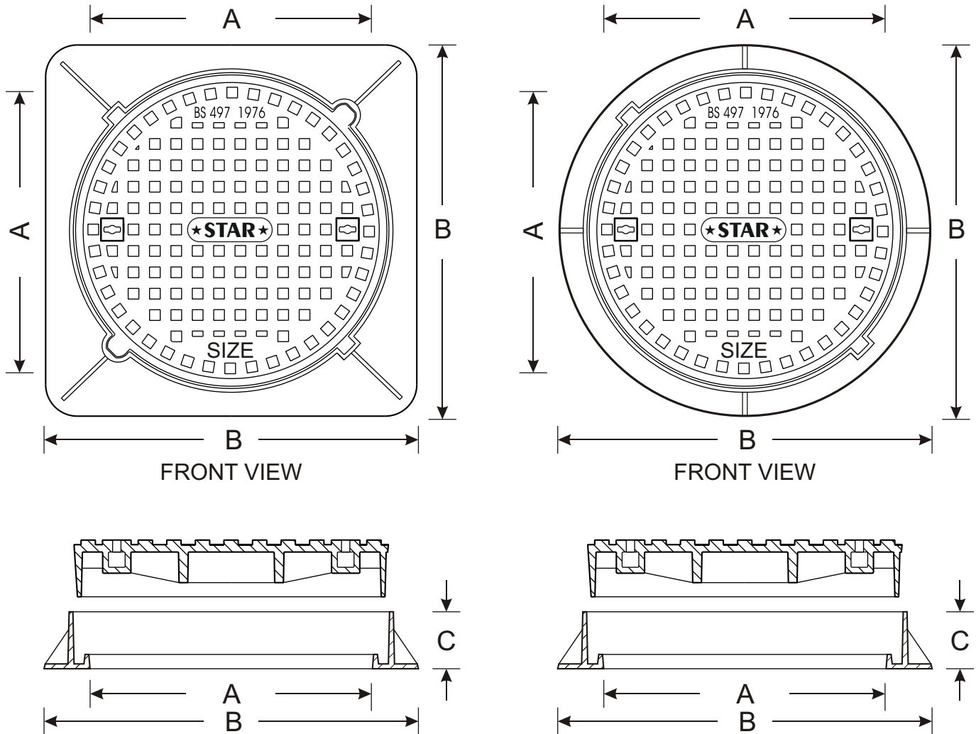
SECTIONAL VIEW OF COVER & FRAME
